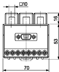
CONVERTER (판형형)
